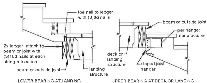
Figure 28 STRINGER BEARING
