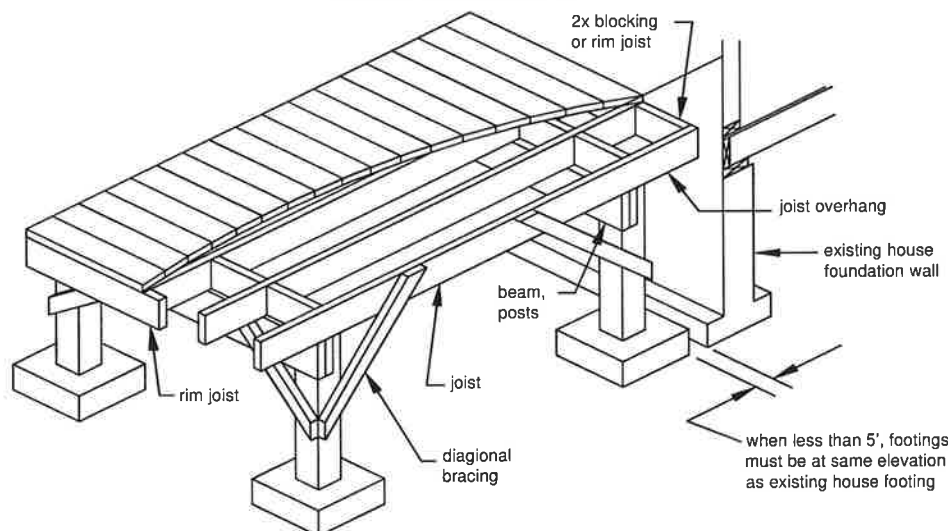
Figure 17 FREE-STANDING DECK
