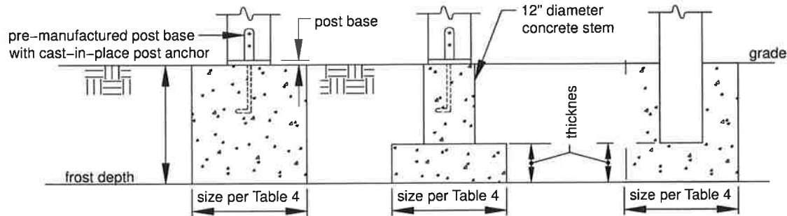
Figure 1 FOOTINGS
