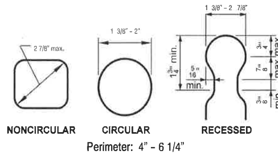
Figure 34 HANDRAIL GRASPABILITY
