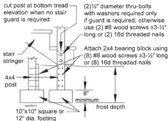
Figure 29 STRINGER BEARING
