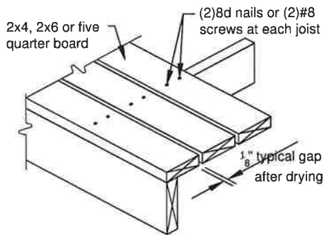
Figure 22 TYPICAL DECKING
