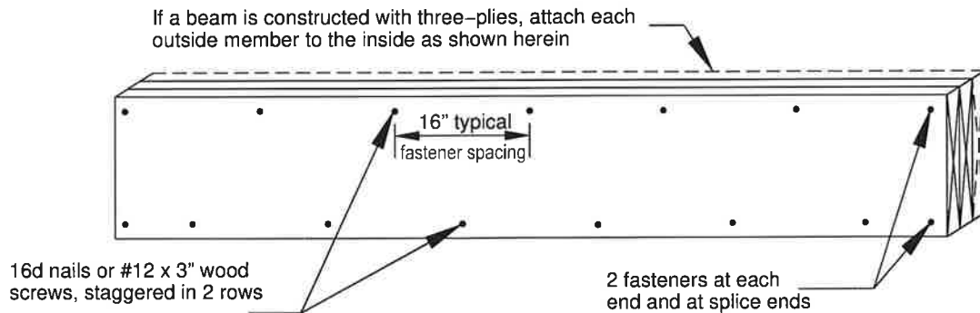
Figure 4 BEAM ASSEMBLY
