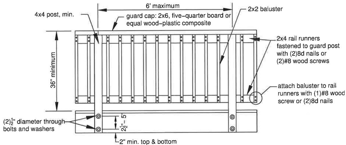
Figure 24 GUARDS
