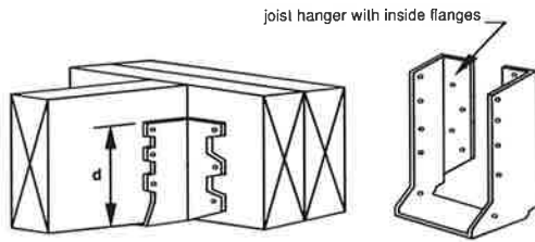
Figure 9 JOIST HANGERS
