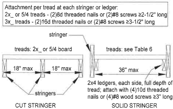
Figure 31 STAIRWAY TREADS
