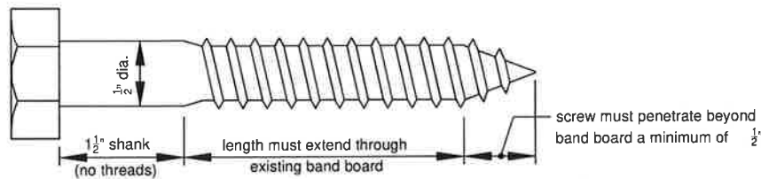
Figure 16 LAG SCREW
