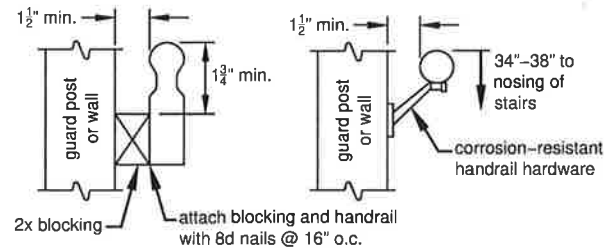
Figure 34 HANDRAIL GRASPABILITY
