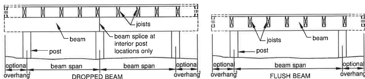
Figure 3 BEAM TYPES
