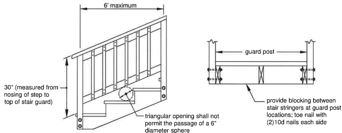
Figure 32 STAIR GUARDS
